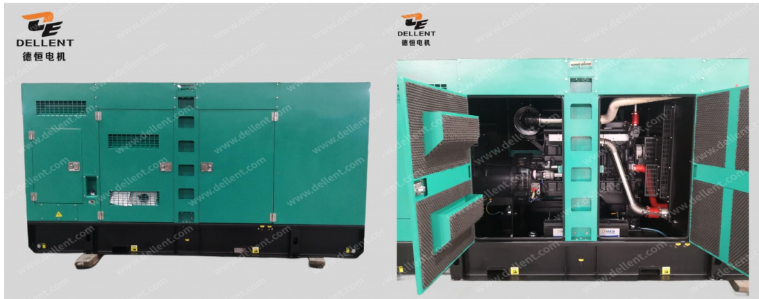
150kVA Diesel Generator Powered by Ricardo Diesel Engine:
